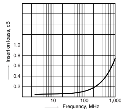
11.-(2) High-frequency characteristics Insertion loss characteristics
