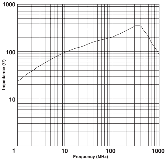
RRH259-128-286
