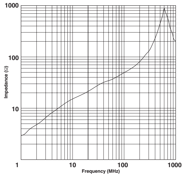
RT120-060-040
