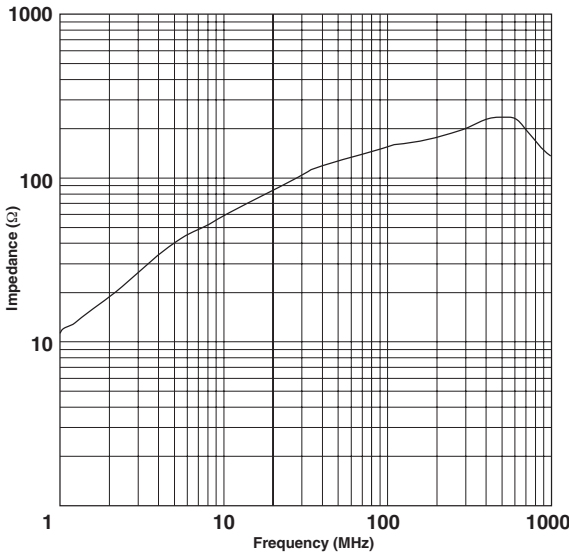
RRH050-015-110
