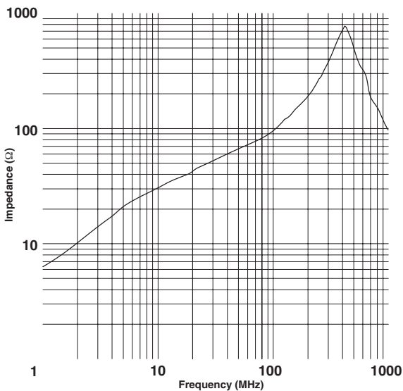
RT406-274-150
