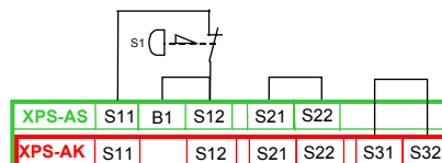
Monitoring of E-stop with 1N/C contact
