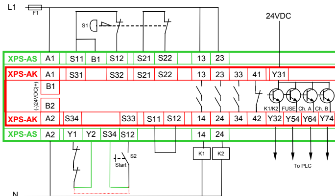
Monitoring of E-stop with 2N/C contacts
