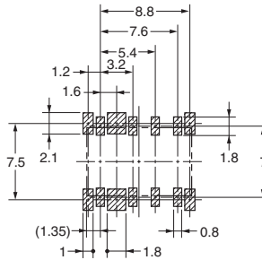
Mounting Dimensions (Top View) Tolerance: \pm 0.1 mm
