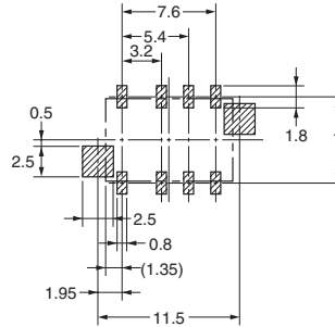
Mounting Dimensions (Top View) Tolerance: \pm 0.1 mm
