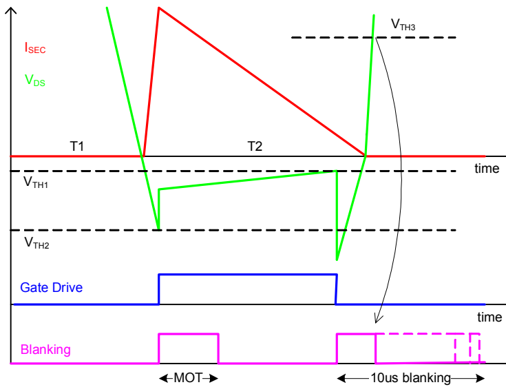
Secondary side DCM/CrCM operation
