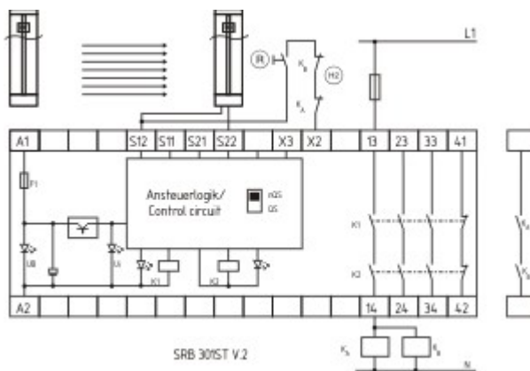
Wiring example
