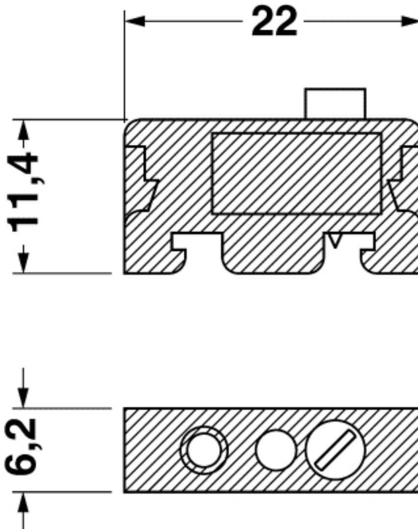
Dimensioned drawing
