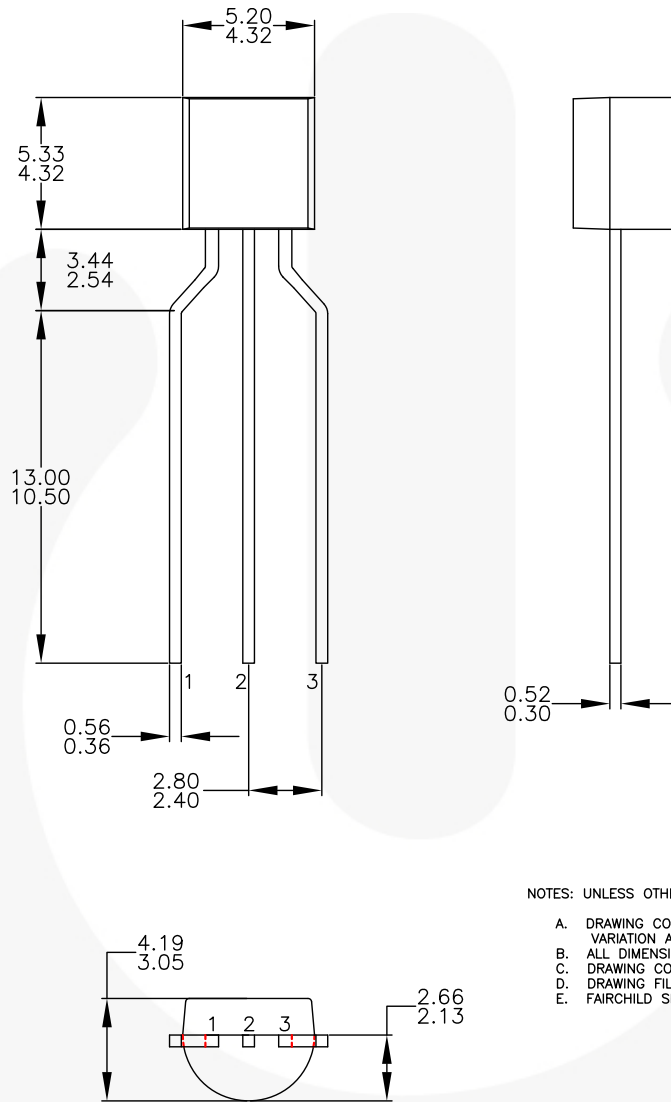
Figure 6. 3-LEAD, TO-92, MOLDED 0.200 IN-LINE SPACING LD FORM (J61Z OPTION) (ACTIVE)
