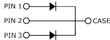
TO-274-3
