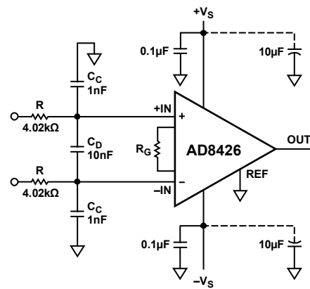
Figure 67. RFI Suppression
