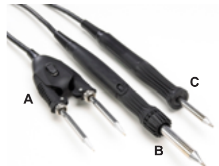
MFR-2200 Series Hand-pieces A. MFR-H4-TW Precision Tweezer B. MFR-H2-ST Soldering Tip C. MFR-H1-SC Soldering Cartridge
