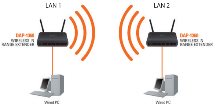
Connecting two separate LANs together through two DAP-1360 units (Wireless PCs cannot access the DAP-1360 units)
