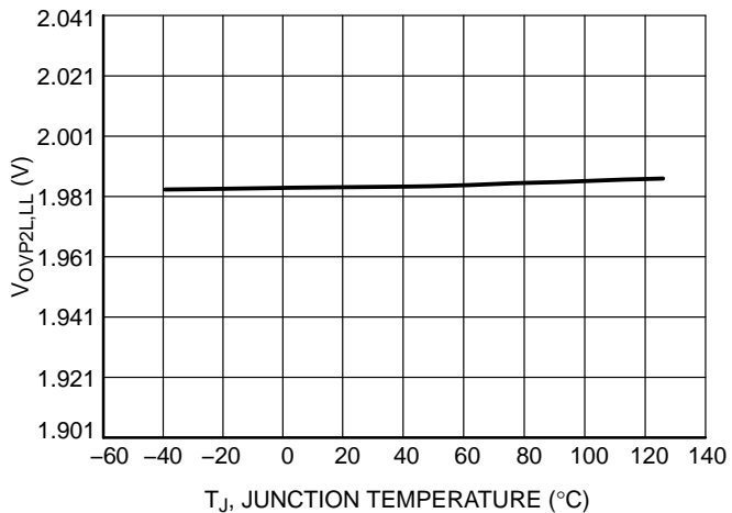
Figure 69. OVP2 Threshold, V CS Falling, K CS = 138, @V REF2 = 1.6 V, (V OVP2(LL) ) vs. Junction Temperature
