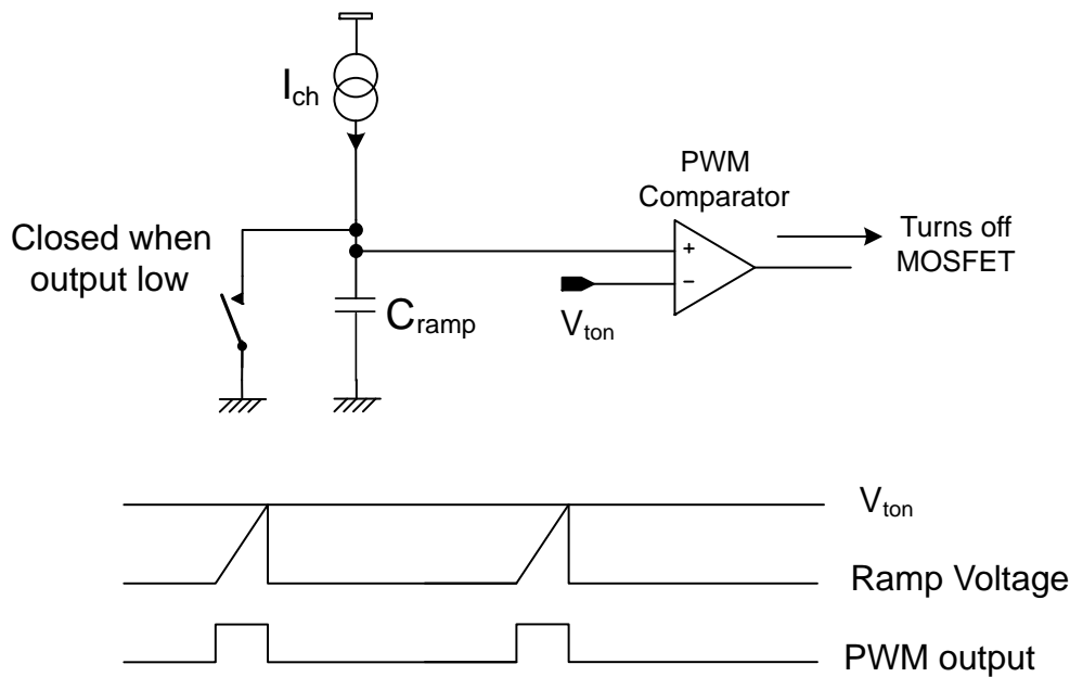
Figure 80. PWM Circuit and Timing Diagram
