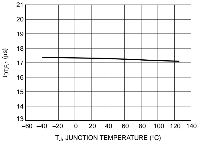
Figure 17. Dead-Time, V_{ctrl} = 0.65\text{ V w/ F Config (}t_{DT,F,1}\text{) vs. Junction Temperature
