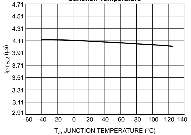
Figure 12. Dead-Time, V_{ctrl} = 0.75 V w/ B Config ( t_{DT,B,2} ) vs. Junction Temperature
