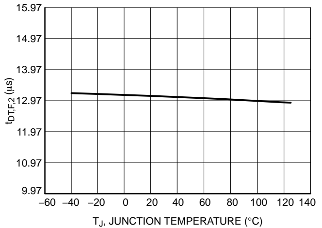
Figure 18. Dead-Time, V_{ctrl} = 0.75\text{ V w/ F Config (}t_{DT,F,2}\text{) vs. Junction Temperature
