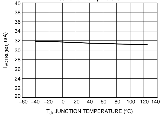
Figure 60. V_{CTRL} Pin Sink Current during BO Condition vs. Junction Temperature
