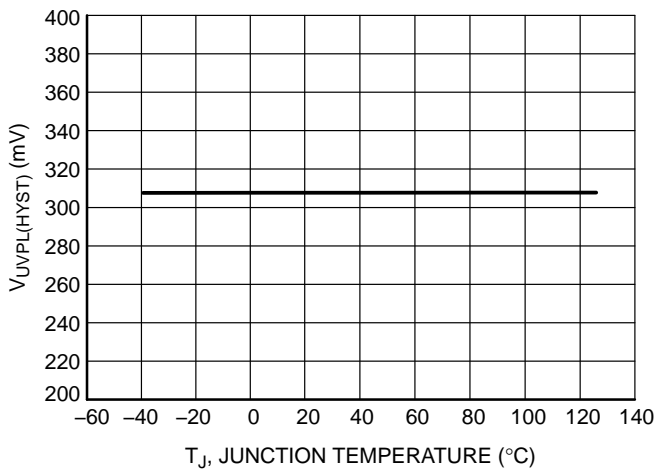
Figure 53. UVP Threshold Hysteresis ( V_{UVPL(HYST)} ) vs. Junction Temperature
