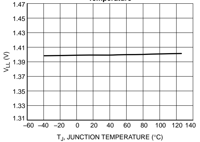
Figure 62. Comparator Threshold for Line Range Detection, V_{LL} vs. Junction Temperature
