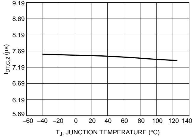
Figure 16. Dead-Time, V_{ctrl} = 0.75\text{ V w/ C Config (}t_{DT,C,2}\text{) vs. Junction Temperature
