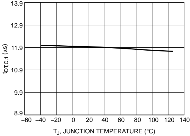
Figure 15. Dead-Time, V_{ctrl} = 0.65\text{ V w/ C Config (}t_{DT,C,1}\text{) vs. Junction Temperature
