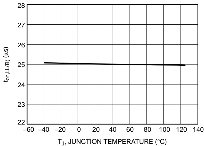
Figure 43. Maximum On Time, avg(V_{CS}) = 0.9 V & V_{ctrl} maximum (CrM) & Low Line for B Version ( t_{on,LL,B} ) vs. Junction Temperature
