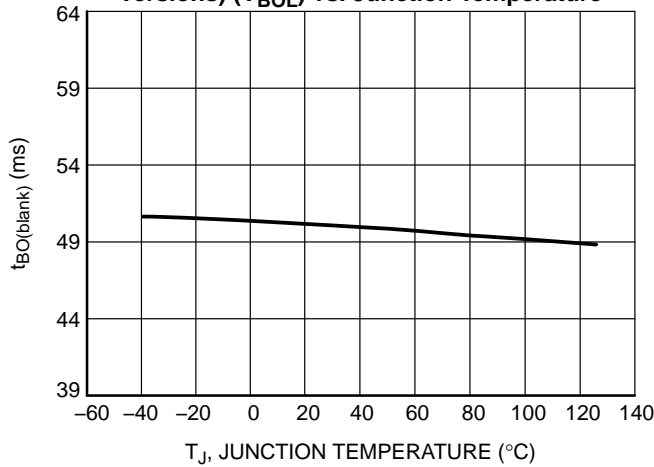
Figure 59. Brown-Out Blanking Time vs. Junction Temperature
