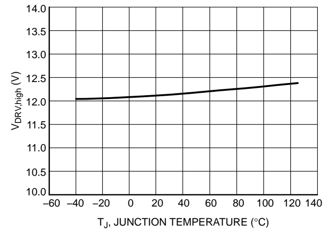
Figure 26. DRV Pin Level @ V_{CC} = 30 V ( R_L = 33 k \Omega & C_L = 1 nF) ( V_{DRV,high} ) vs. Junction Temperature
