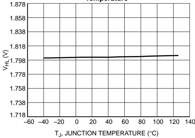
Figure 61. Comparator Threshold for Line Range Detection, V_{HL} vs. Junction Temperature
