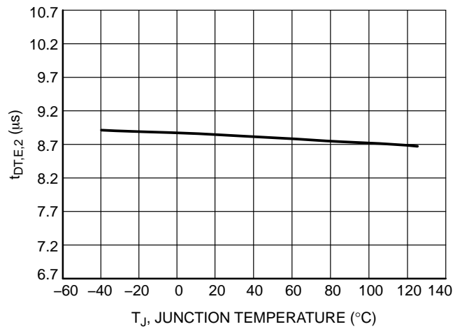
Figure 14. Dead-Time, V_{ctrl} = 0.75 V w/ E Config ( t_{DT,E,2} ) vs. Junction Temperature
