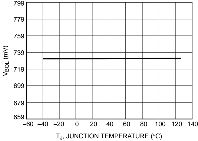
Figure 57. Brown-Out Threshold, V_{BO(L)} vs. Junction Temperature
