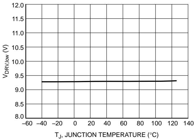
Figure 25. DRV Pin Level for V_{CC} = V_{CC,off} + 200 mV (10-k \Omega Resistor between DRV and GND) ( V_{DRV,low} ) vs. Junction Temperature
