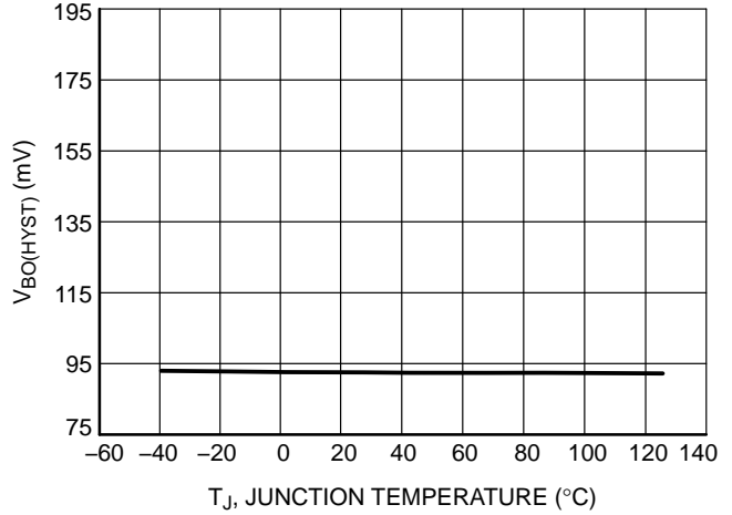
Figure 58. Brown-Out Comparator Hysteresis vs. Junction Temperature
