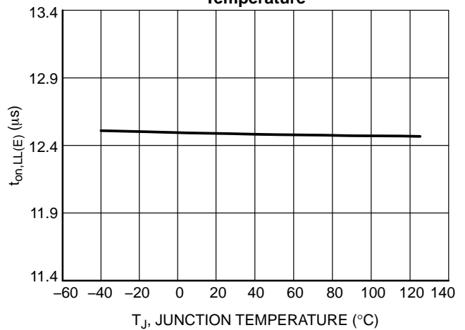
Figure 44. Maximum On Time, avg(V_{CS}) = 0.9 V & V_{ctrl} Maximum (CrM) & Low Line for E Version ( t_{on,LL,E} ) vs. Junction Temperature
