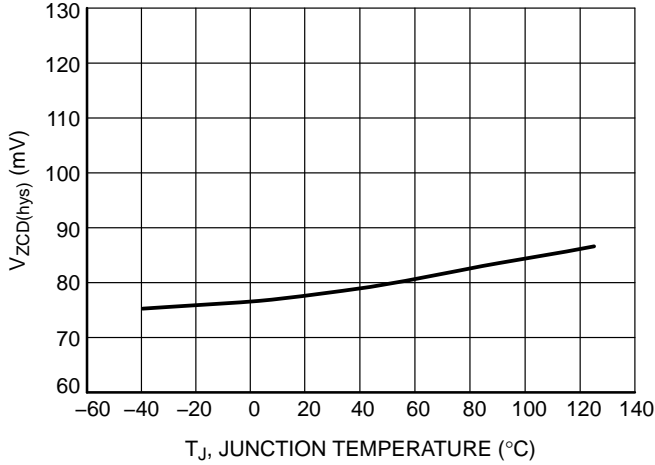
Figure 39. Hysteresis of the Zero Current Detection Comparator ( V_{ZCD(hyst)} ) vs. Junction Temperature
