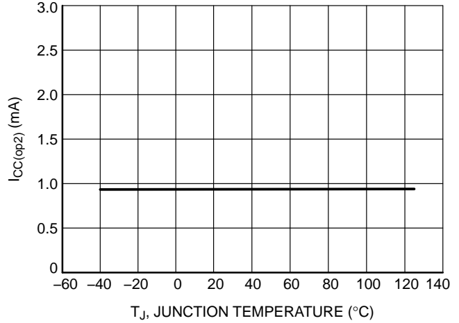
Figure 10. Operation Consumption, 50-kHz Switching, No Load on DRV ( I_{CC,op2} ) Pin vs. Junction Temperature
