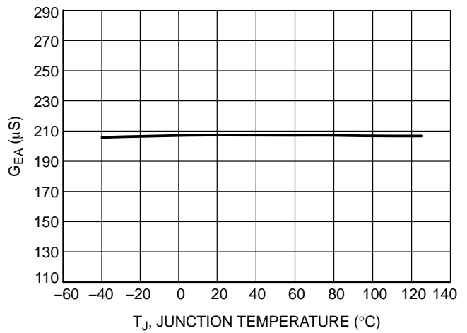
Figure 32. Error Amplifier Transconductance ( G_{EA} ) vs. Junction Temperature
