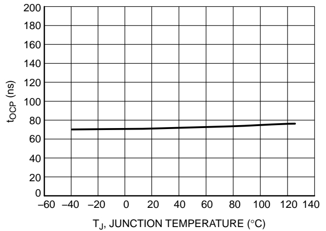
Figure 36. Over-Current Protection Delay from V CS/ZCD > V CS(th) to DRV Low (dV CS/ZCD / dt = 10 V/µs) (t OCP ) vs. Junction Temperature
