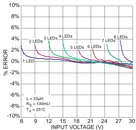
Fig. 28 LED Current Deviation vs. Input Voltage
