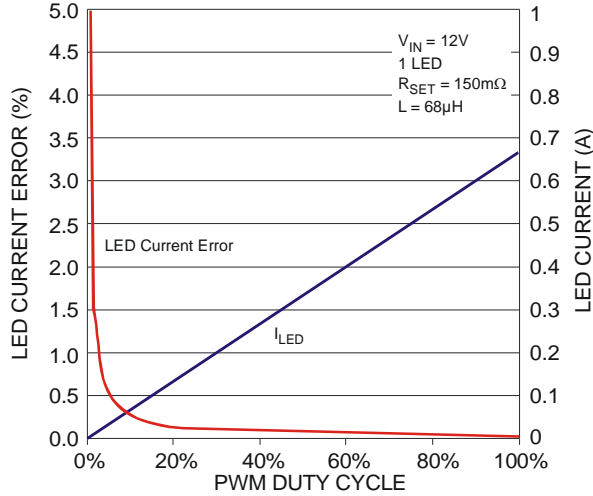
Fig. 7 I_{LED} vs. PWM Duty Cycle
