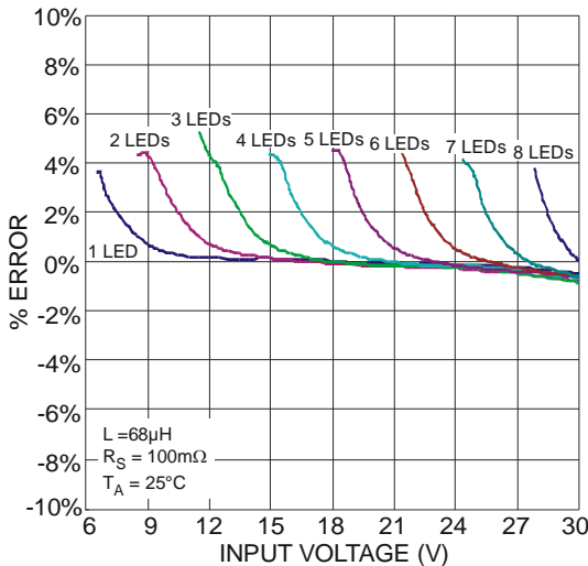
Fig. 26 LED Current Deviation vs. Input Voltage
