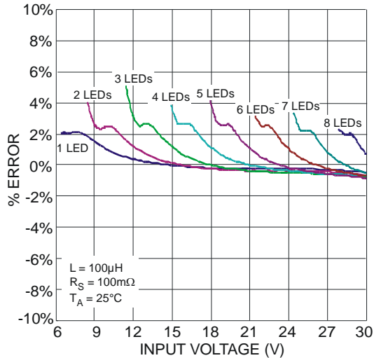
Fig. 24 LED Current Deviation vs. Input Voltage
