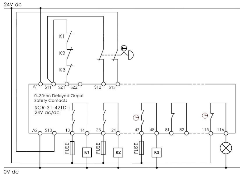
Fig.1 SCR-31-42TD-i, Dual Channel, E-Stop, Auto Reset
