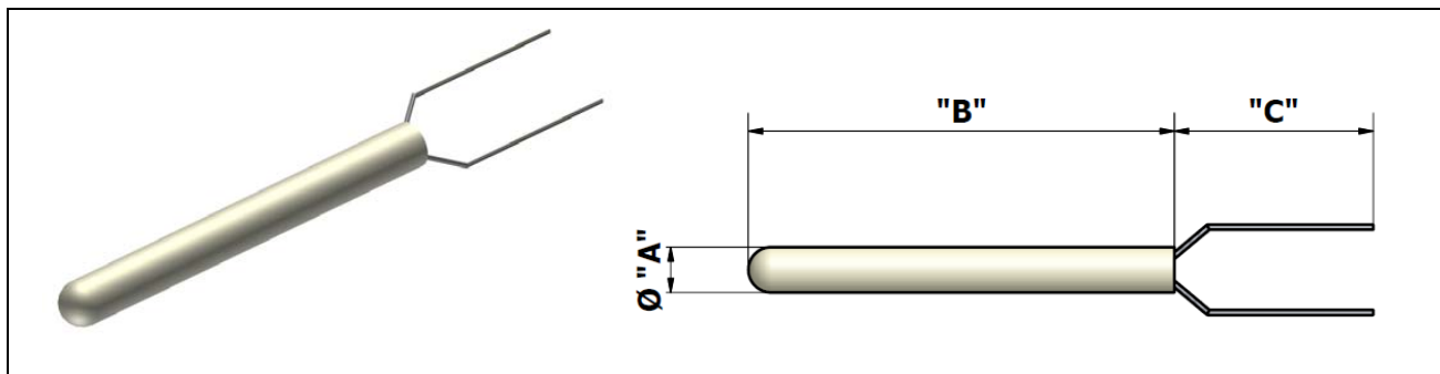
WOUND PT100Ω THERMIC ELEMENT
