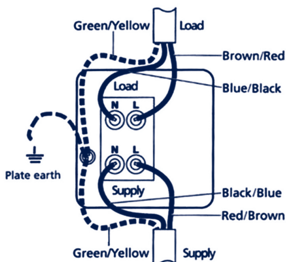
Wiring diagram
