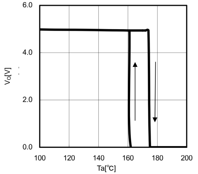
Figure 28. TSD ( I_o=0mA )
