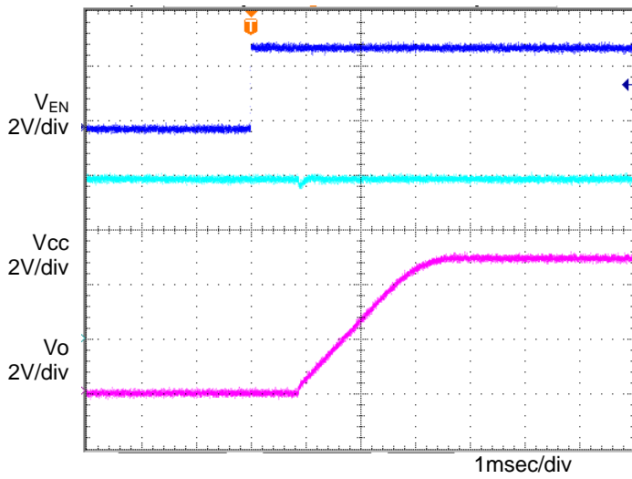
Figure 17. Input sequence 2 C o =1μF, T a =105°C
