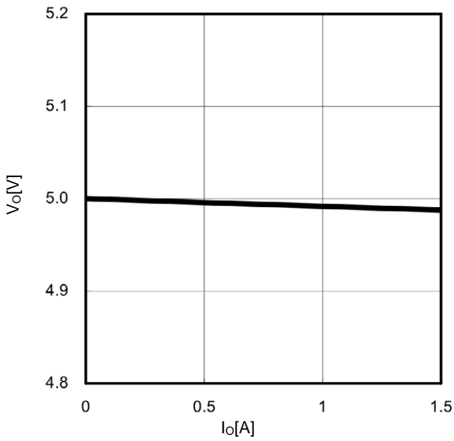
Figure.25. I_O - V_O
