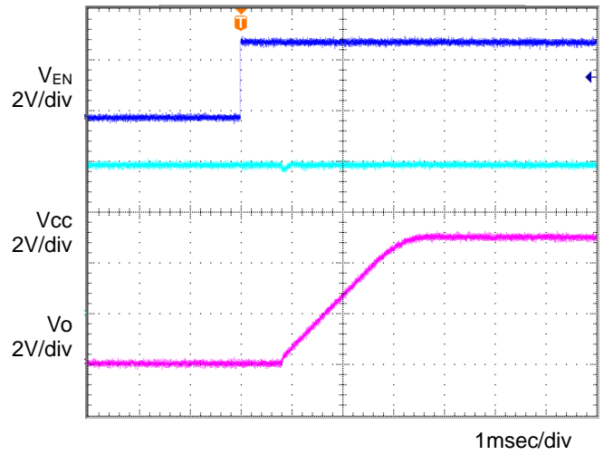
Figure 16. Input sequence 2 C o =1μF, T a =25°C
