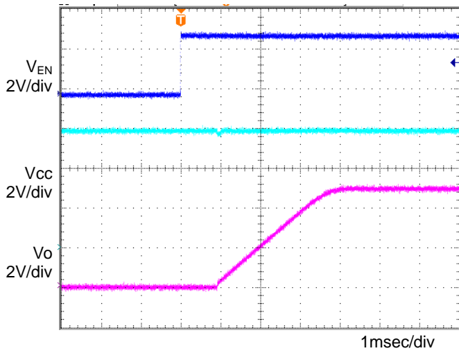
Figure 15. Input sequence 2 C o =1μF, T a =-40°C
