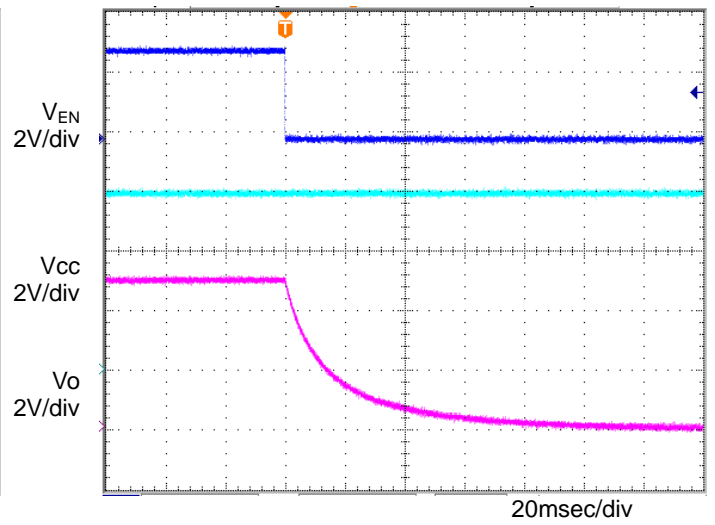
Figure 18. OFF sequence 2 C o =1μF, T a =-40°C
